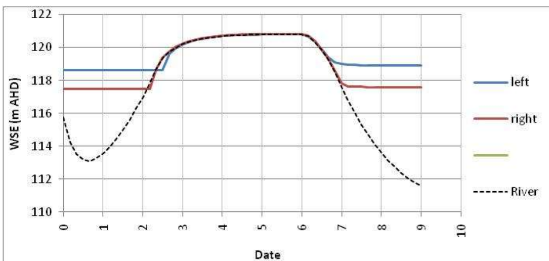
Figure 7-7 Model E2 downstream extraction line 60,000 ML/d
