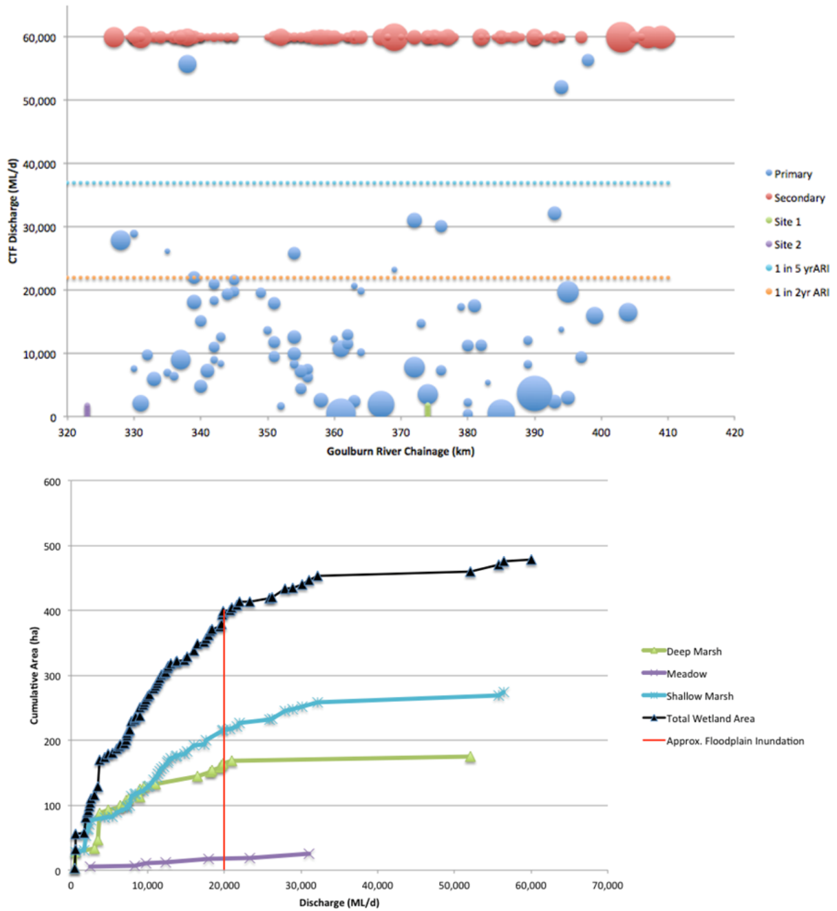
Figure 5: Example outputs of the wetland CTF assessment for Reach 1: CTF levels for selected wetlands (above) and cumulative wetland area with increasing discharge (below).
