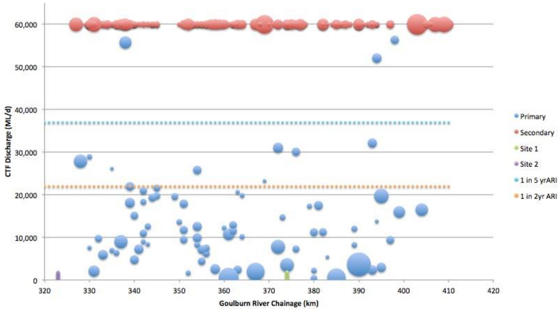
Figure 12: Reach 1 wetlands with primary connections (blue) to the Goulburn River and their CTF discharges relative to their river chainage. Wetlands with secondary connections (red) are displayed with a nominal CTF, as these were not available. Bubble size represents relative wetland size.
