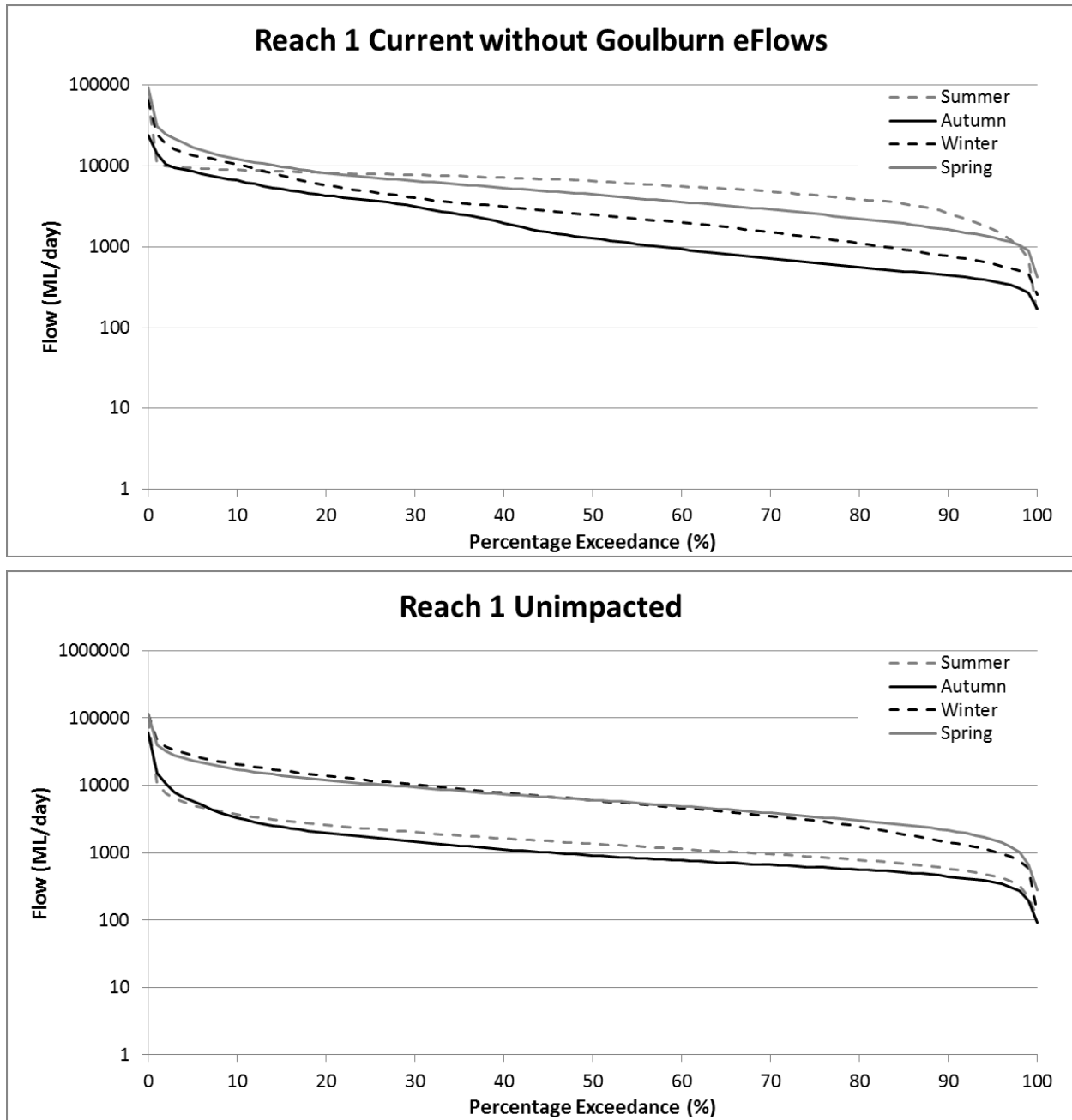
Figure 2: Flow duration curves showing seasonal patterns for modelled current and unimpacted conditions in Reach 1.
