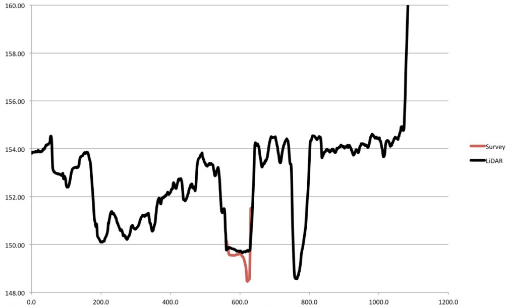
Figure 10: Cross-section 2325m (Site 1) relative to elevation (mAHd) showing multiple channels. This illustrates how the depth of the main channel captured by LiDAR (black line) is obscured by water in the bed of the channel, when compared to channel depth from one of the repeat surveys (red) conducted in 2014. This section indicates water depth at the time of survey as approximately 1.2m.
