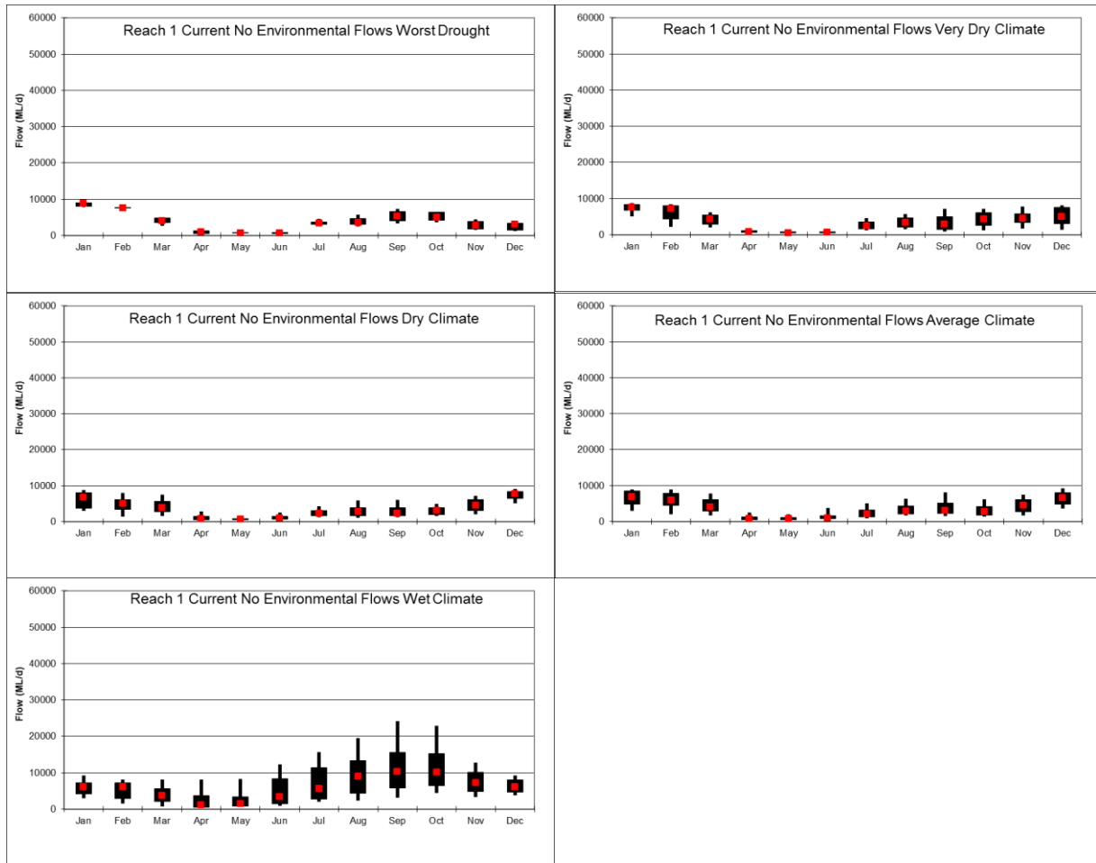
Figure 3: Plots of mean daily flow for the modelled current flow regime (with environmental releases omitted) for Reach 1 under various climatic conditions. Dots in centre of boxes are median values, boxes span the 25th to 75th percentiles, while whiskers span the 5th to 95th percentiles.
