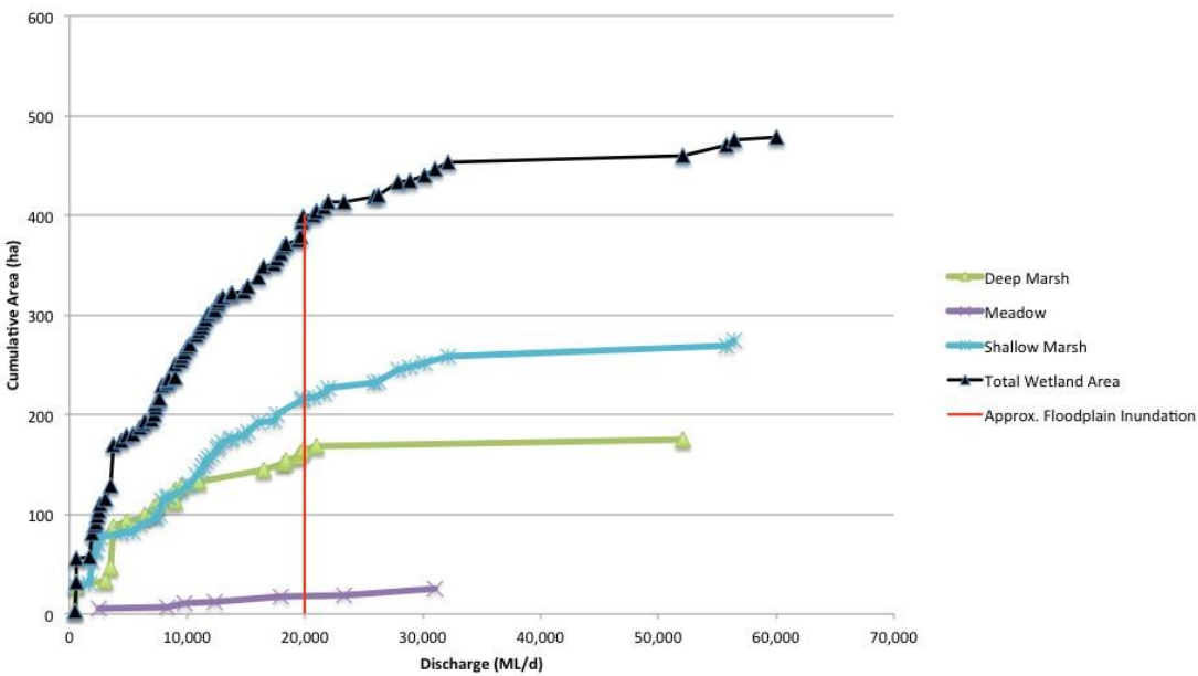
Figure 13: Reach 1 cumulative area of wetlands relative to the discharge at which those wetlands are engaged for all wetlands (dark blue) and by type: Shallow Marsh (light blue), Deep Marsh (green) and Meadow (purple). Approximate floodplain inundation discharge is labelled in red.
