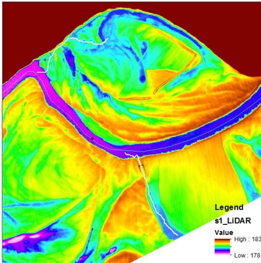
Figure 9: Example of connector string (thin white line) between the Goulburn River and wetlands e.g. 809825 to top of picture. Colour graduations represent elevation (mAHD) from low water level during time of survey (178m) to points higher than 183m as per the legend.
