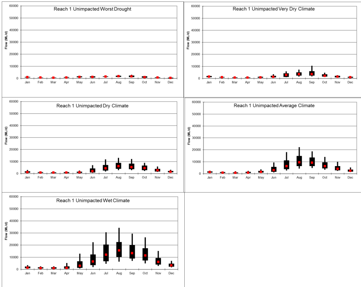
Figure 4: Plots of mean daily flow for the modelled unimpacted flow regime for Reach 1 under various climatic conditions. Dots in centre of boxes are median values, boxes span the 25 th to 75 th percentiles, while whiskers span the 5 th to 95 th percentiles.
