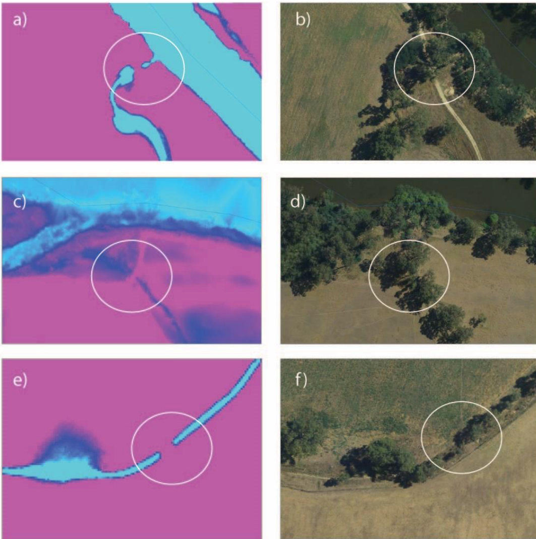
Figure 15: Significant changes to CTF levels occurs as a result of direct modification in many ways such as through: road construction (a-b, LiDAR-aerial image), the construction of levees to reduce inundation of land (c/d) and cattle tracks (e-f). In the LiDAR images (left) light blue represents low elevations and pink the highest.
