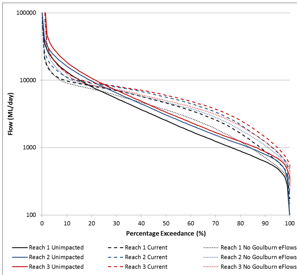
Figure 8: Flow duration curve for the whole period of record for each reach
