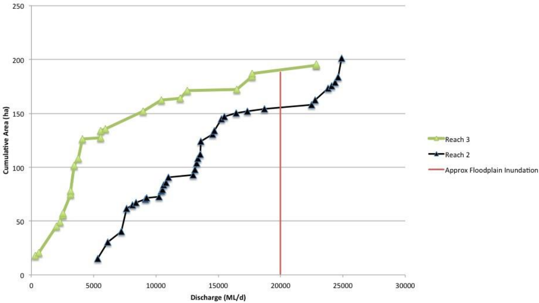
Figure 14: Reach 2 and 3 cumulative area of wetlands relative to the discharge at which those wetlands are engaged for all wetlands assessed. Approximate floodplain inundation discharge is labelled in red.
