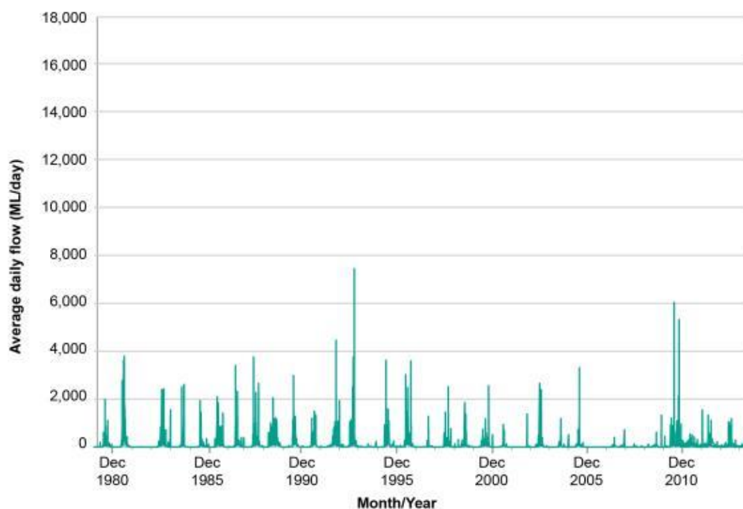
Figure A6 Average daily water flow in Home Creek at Yarck (gauging station 405274), December 1980 – December 2013
