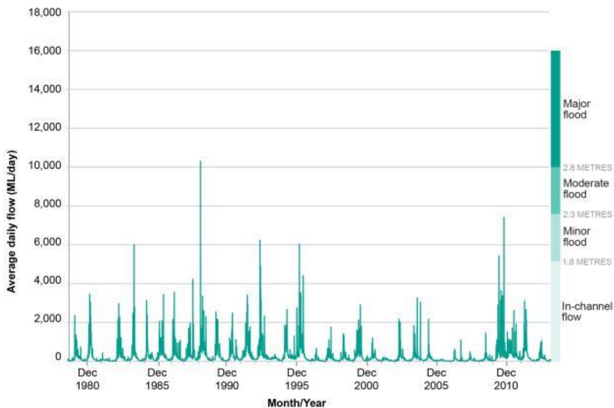
Figure A7 Average daily water flow near Yea at Devlins Bridge (gauging station 405217), December 1980 – December 2013
