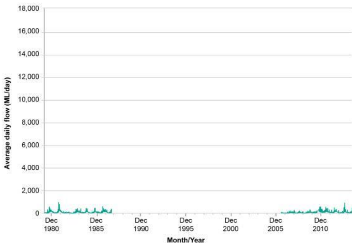
Figure A3 Average daily water flow in Snobs Creek at Snobs Creek hatchery (gauging station 405257), December 1980 – December 2013
