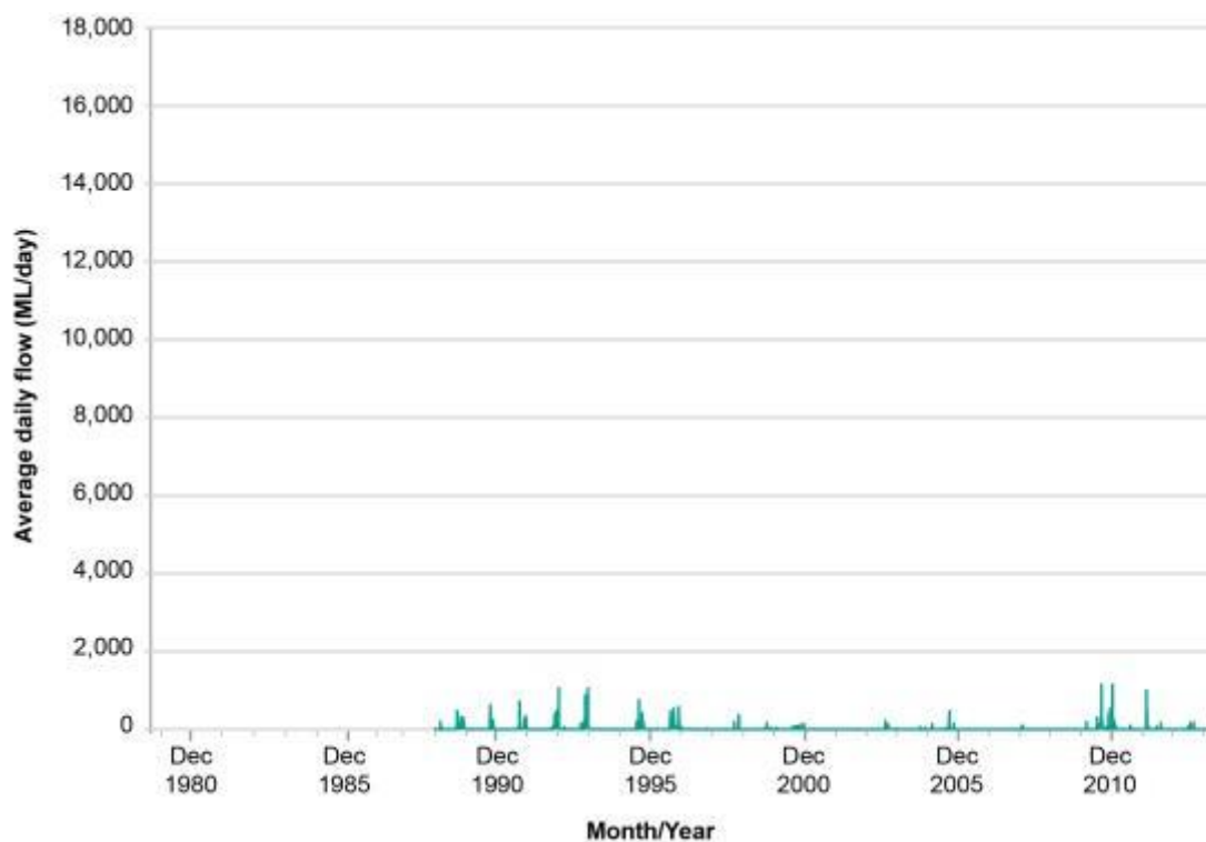
Figure A11 Average daily water flow in Whitehead Creek (gauging station 405273), December 1980 – December 2013
