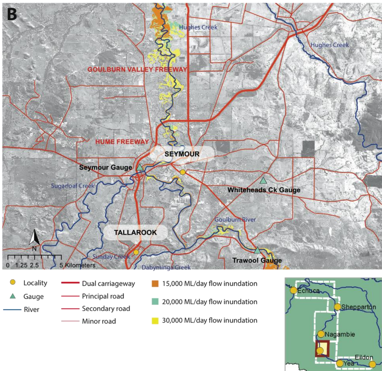
Figure 20 a and b Flow footprints for flows of 12,000, 15,000 and 20,000 megalitres (ML)/day between Ghin Ghin and Mitchellstown
