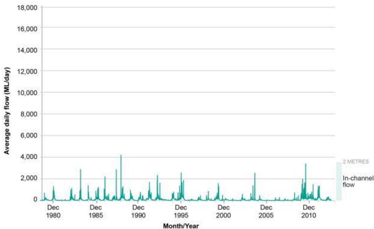
Figure A8 Average daily water flow in King Parrot Creek at Flowerdale (gauging station 405231), December 1980 – December 2013
