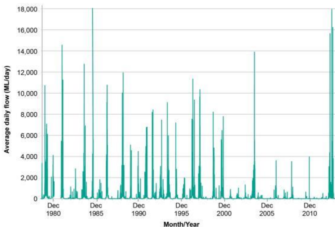
Figure A10 Average daily water flow in Sugarloaf Creek at Ash Bridge (gauging station 405240), December 1980 – December 2013
