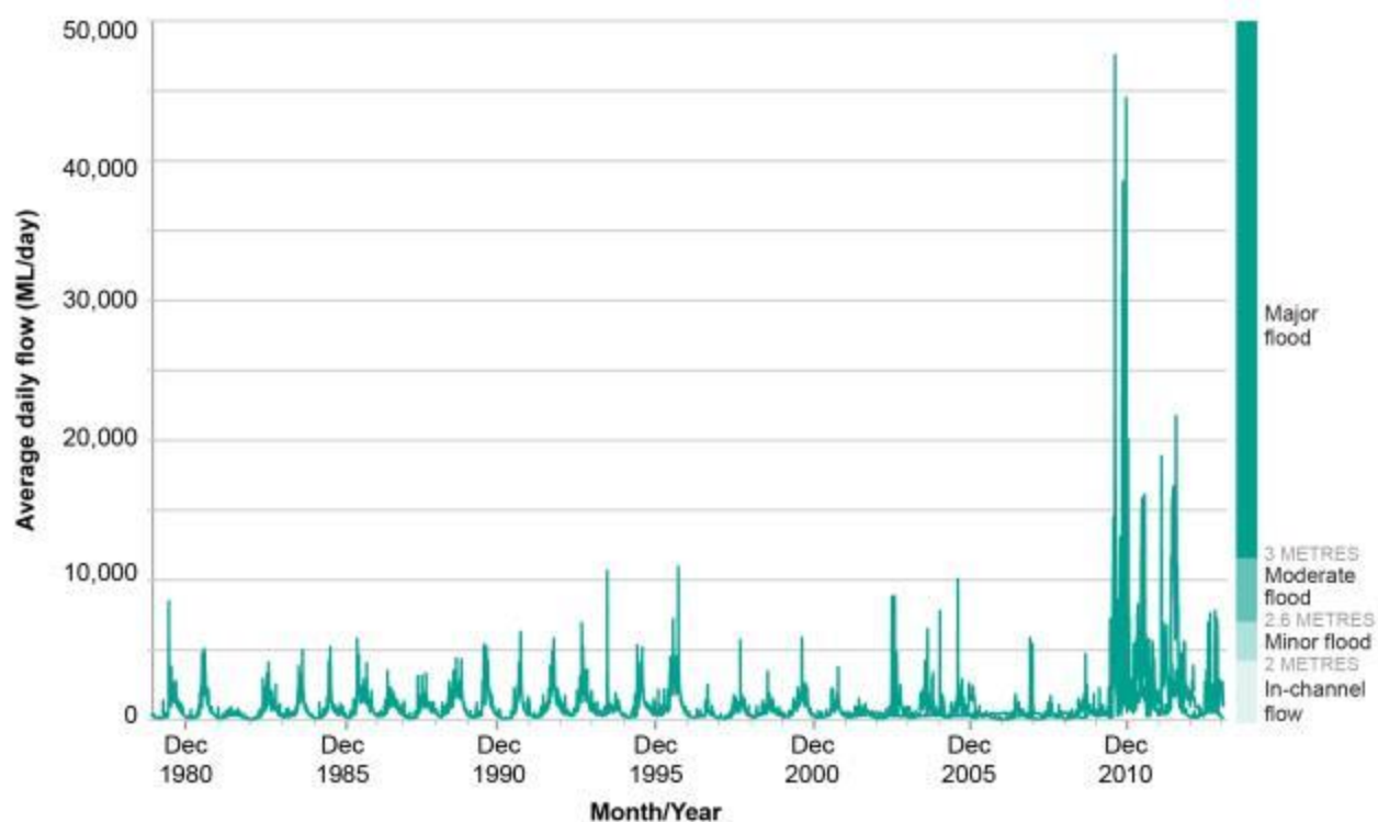
Figure A5 Average daily water flow in Acheron River at Taggerty (gauging station 405209), December 1980 – December 2013
