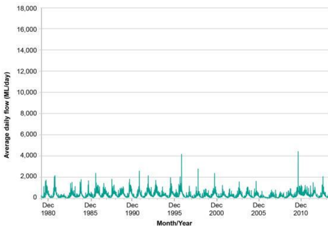
Figure A4 Average daily water flow in Rubicon River (gauging station 405241), December 1980 – December 2013
