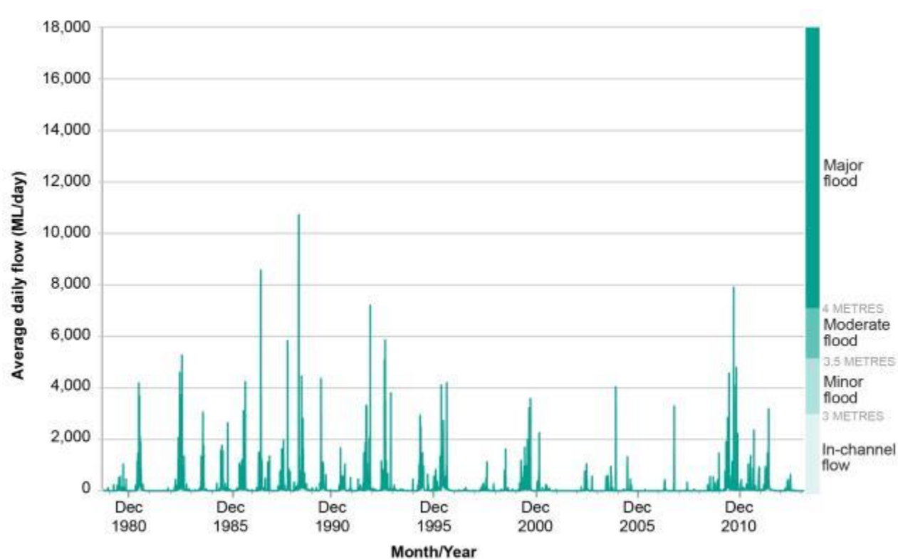
Figure A9 Average daily water flow in Sunday Creek at Tallarook (gauging station 405212), December 1980 – December 2013
