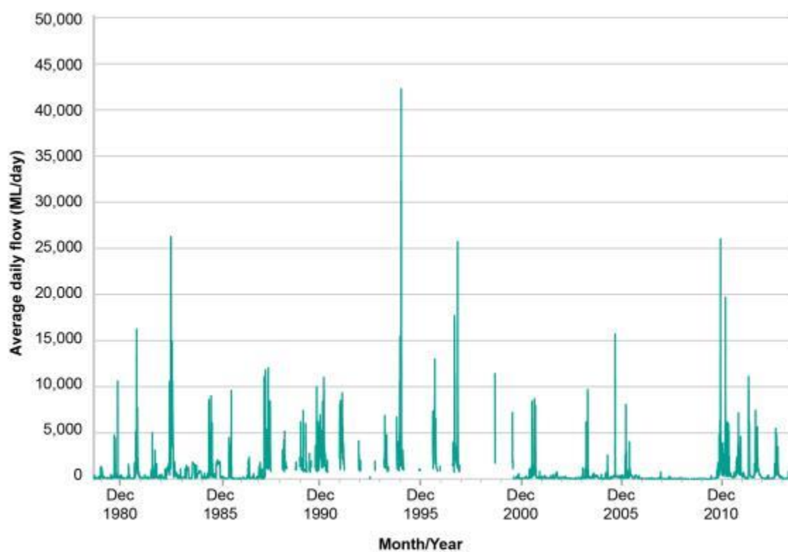
Figure A14 Average daily water flow in Broken River at Orrvale (gauging station 404222), December 1980 – December 2013
