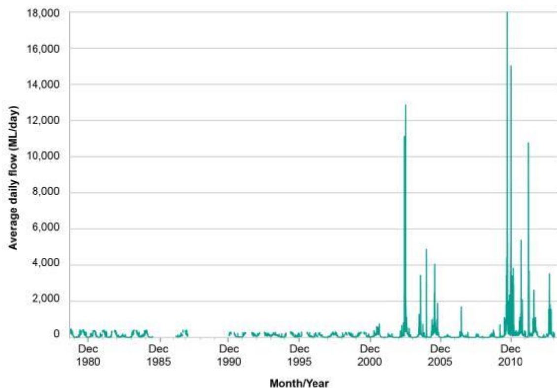
Figure A13 Average daily water flow in Seven Creeks Kialla West (gauging station 405269), December 1980 – December 2013
