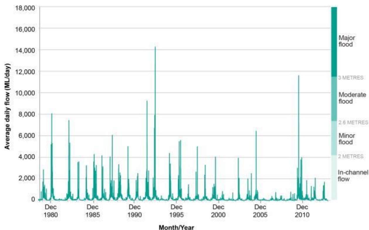
Figure A12 Average daily water flow in Hughes Creek at Tarcombe (gauging station 405228), December 1980 – December 2013
