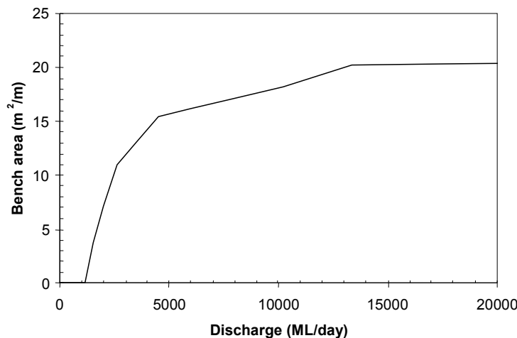
Figure 37: Bench area at Murchison (using model results from the 2003 environmental flow study)
